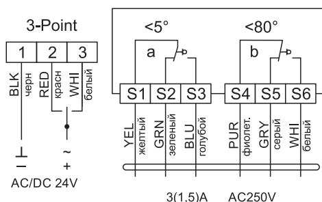
RLF03-220S(H), RLF05-220S(H)
